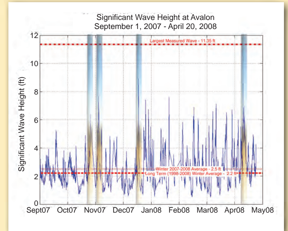
Figure 2: Significant wave height measured at Avalon between September 1, 2007 and April 20, 2008.
